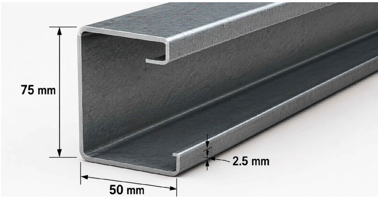
Purlin : 75 × 50 × 2.5 mm
