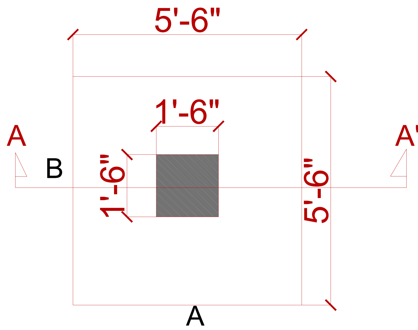
DETAIL - A PLAN of FOOTING(AXB) (FOR DETAILS REFER TABLE(1)) Note - a & b are dimensions of column
