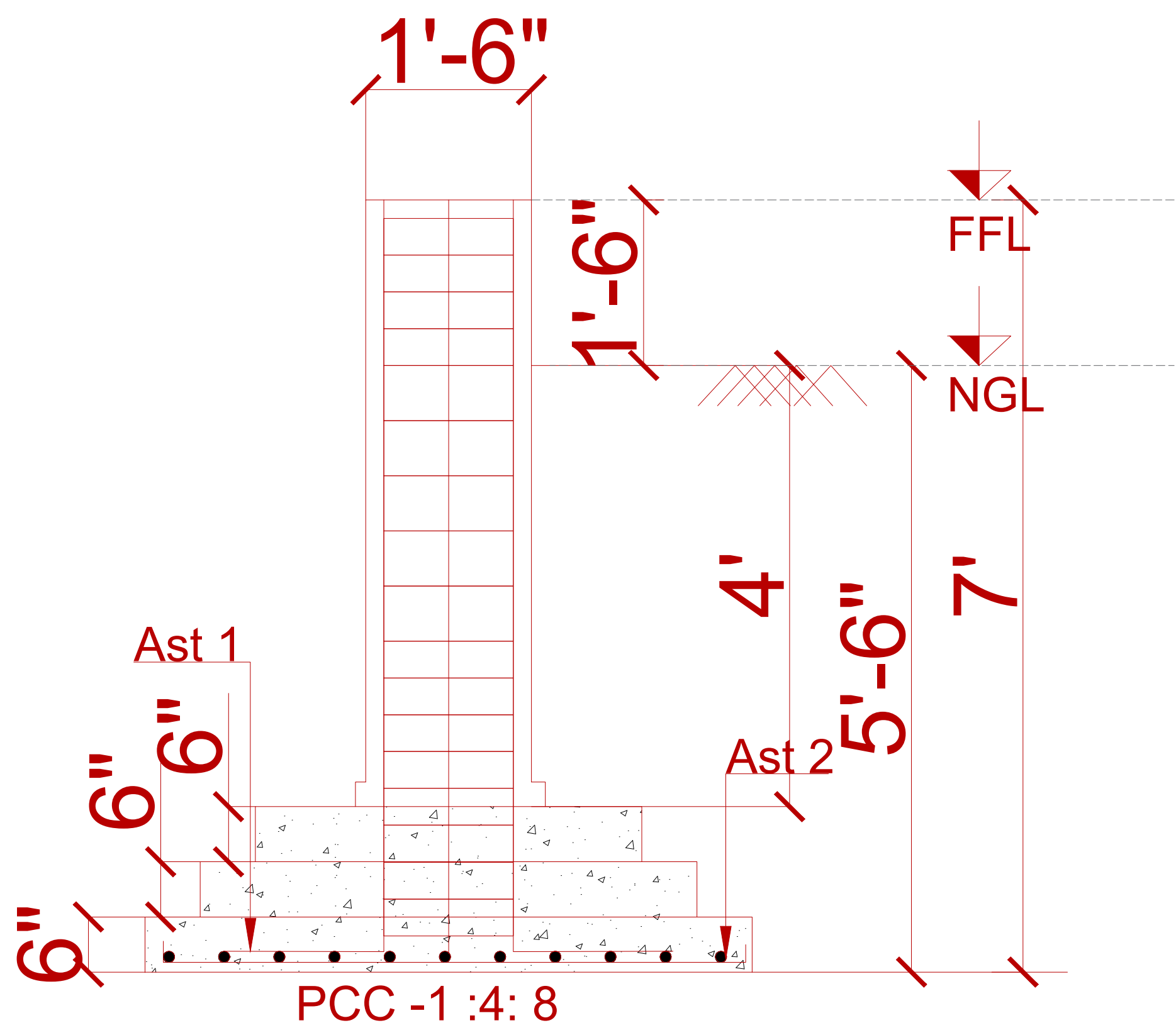
SECTION AA'
