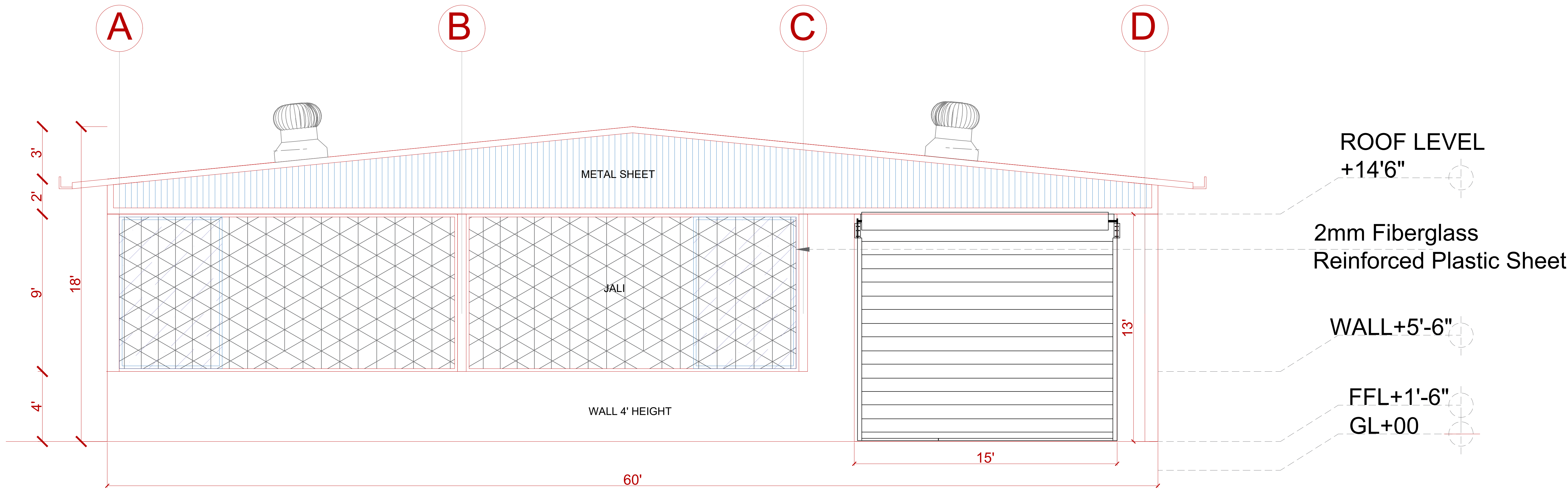
FRONT ELEVATION
