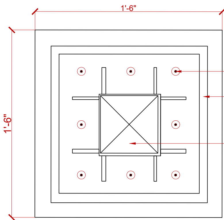
DETAIL A
