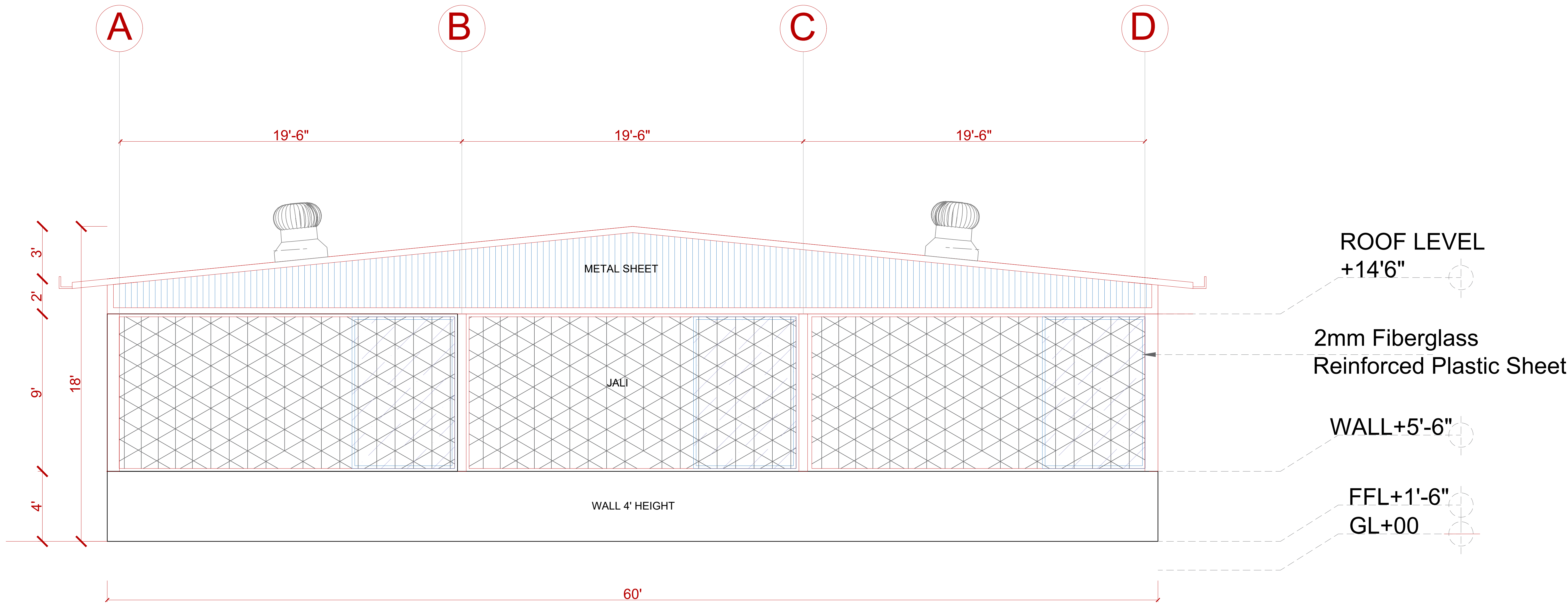
REAR ELEVATION
