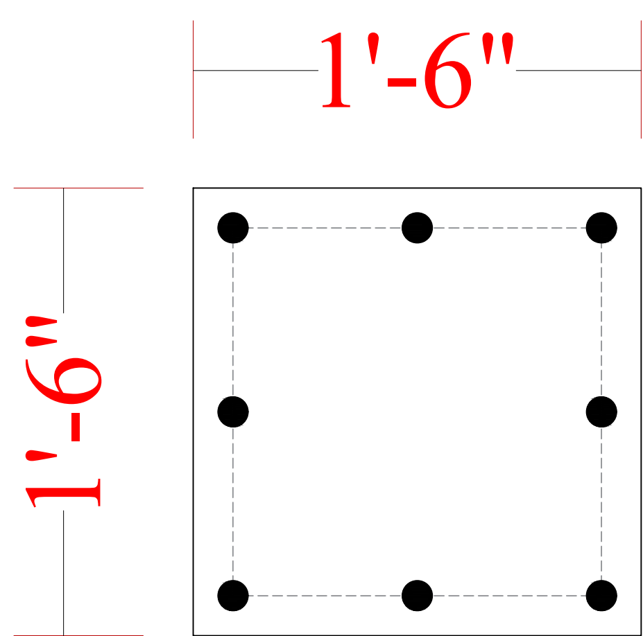
DETAIL B COLUMN REINFORCEMENT PLAN C1
