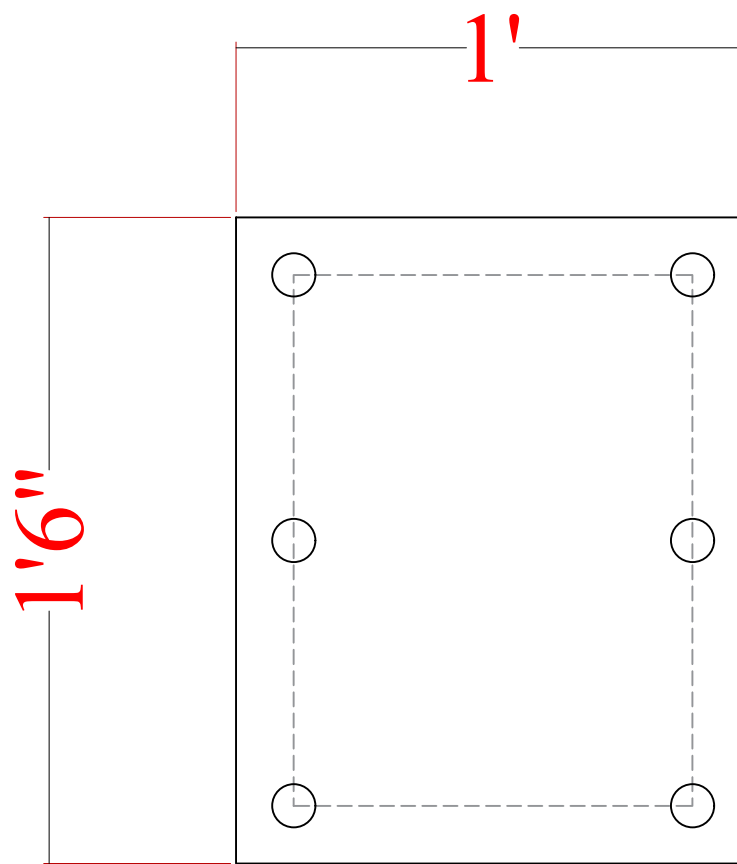
PLINTH BEAM PLAN PB: 16# - 6Nos STIRRUPS- 8#@6"c/c
