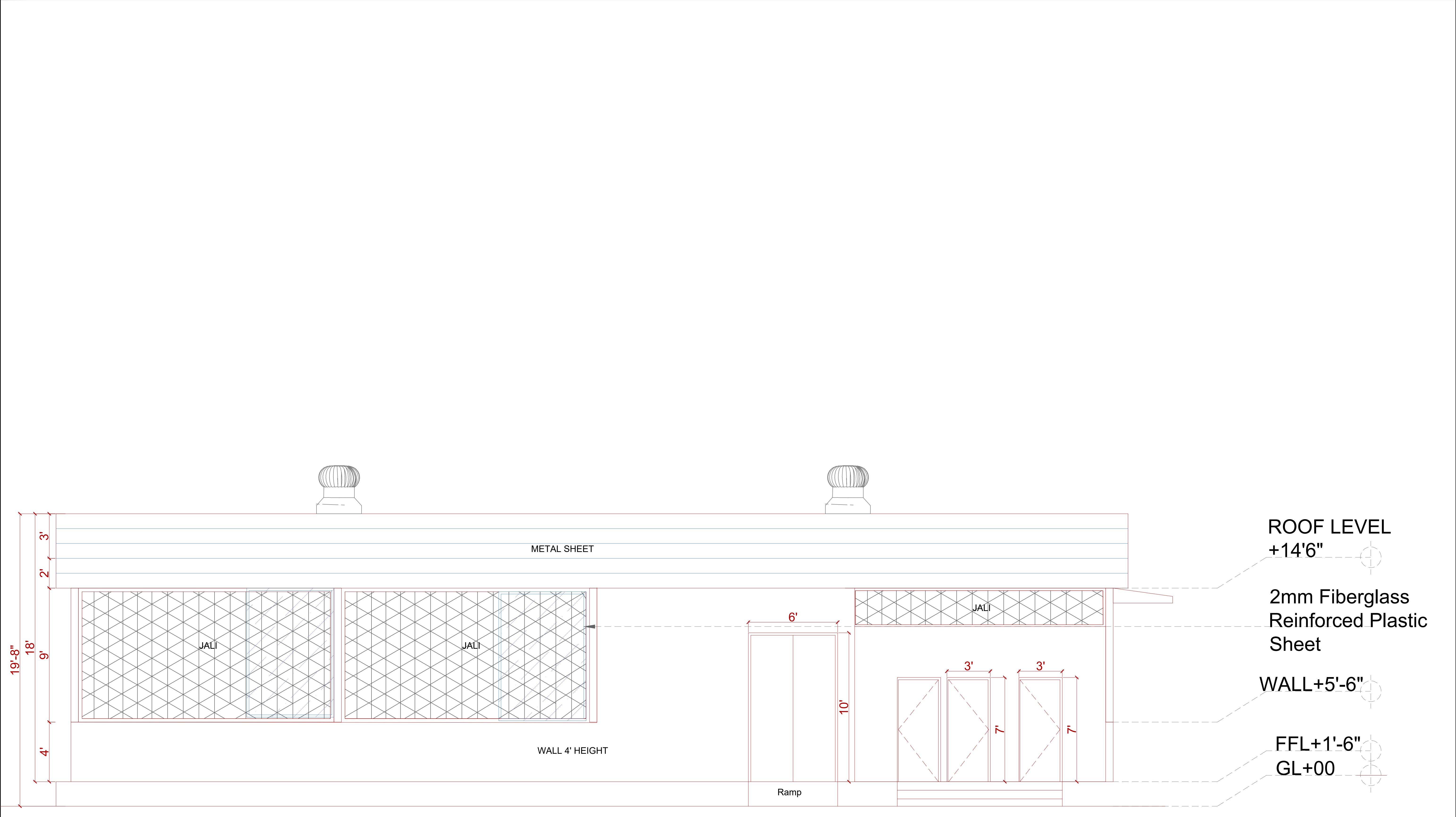
LEFT SIDE ELEVATION
